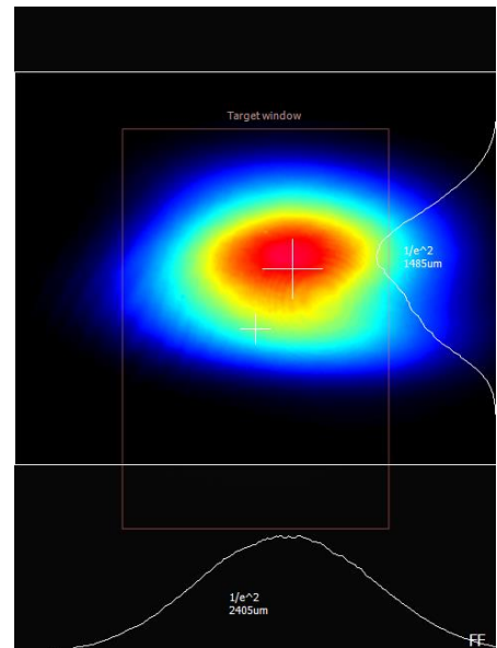
Typical far field (1 m from output aperture) beam profile. Non-circularized beam of a 0830 nm direct diode laser.
