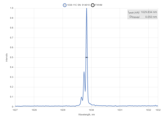
Typical spectrum of 1030 nm passive Q-Switch DPSS laser. Measured with 20 pm resolution.
